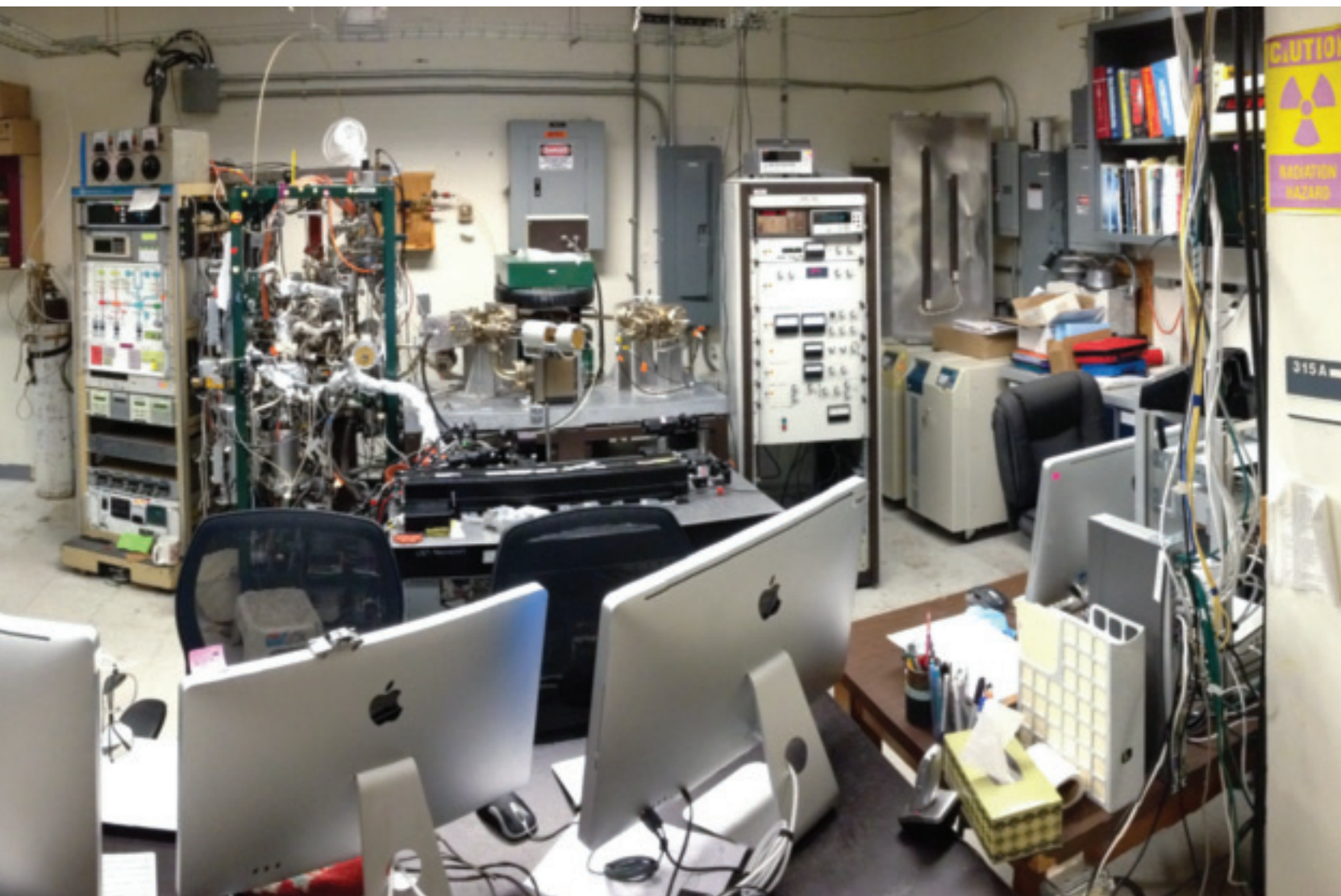
Noble gas mass spectrometry laboratory at the New Mexico Bureau of Mines (courtesy of Dr. Matt Heizler).
